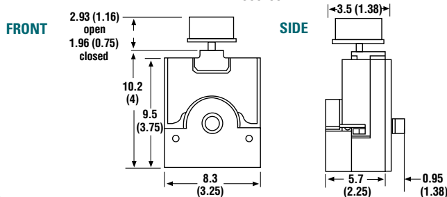
Dimensional Drawings cm (in.) 77390-00
